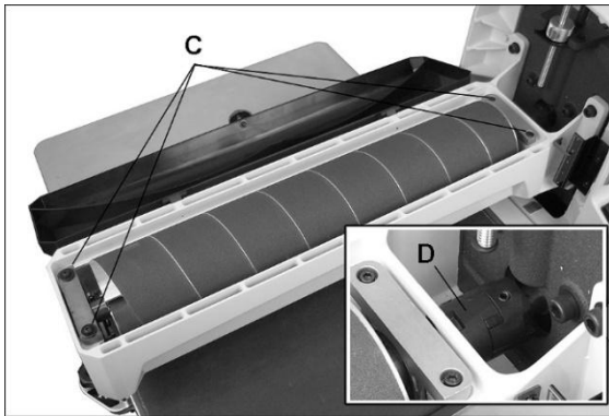
Figure 10-2: drum removal
