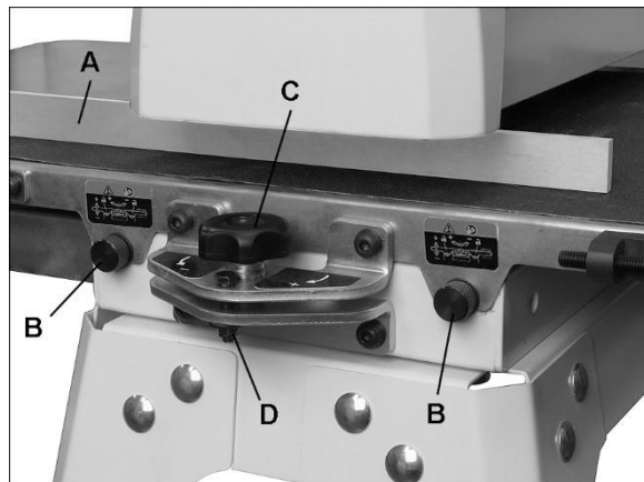
Figure 8-3: drum alignment
