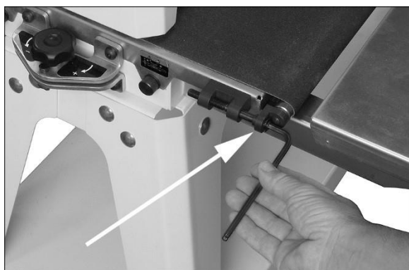
Figure 8-2: belt tension adjustment
