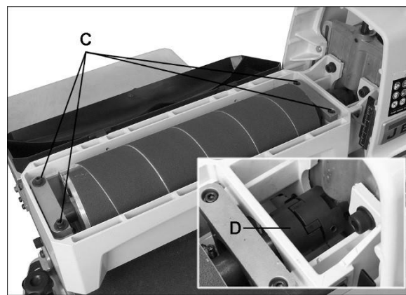
Figure 10-2: drum removal
